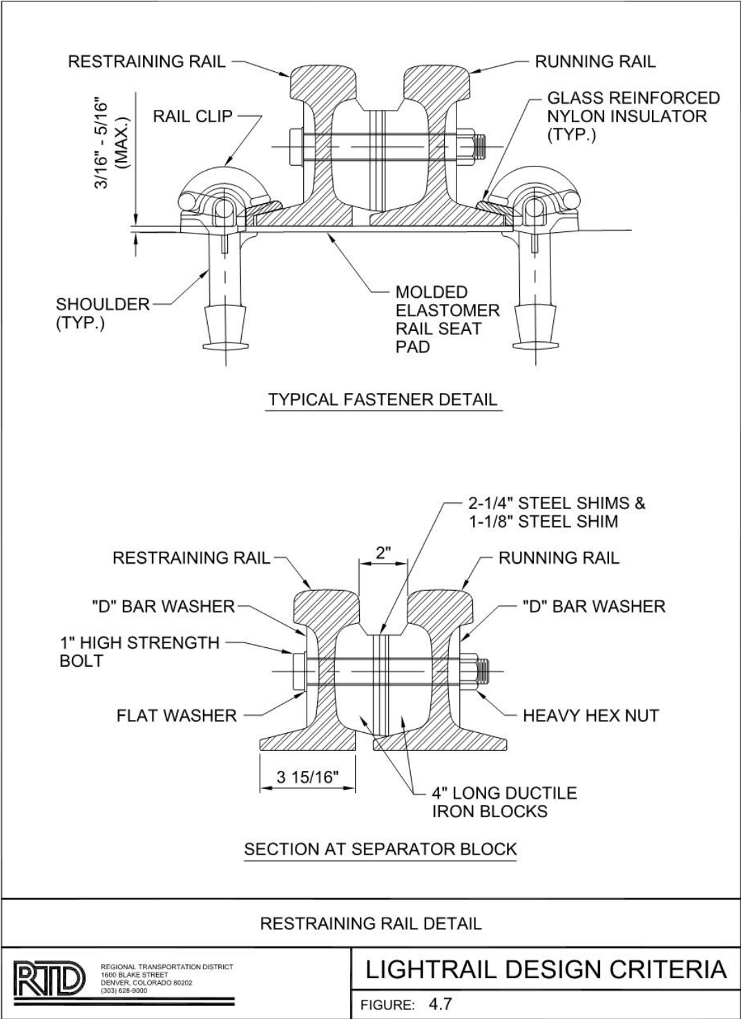
FIGURE 4.7 - RESTRAINING RAIL DETAIL
