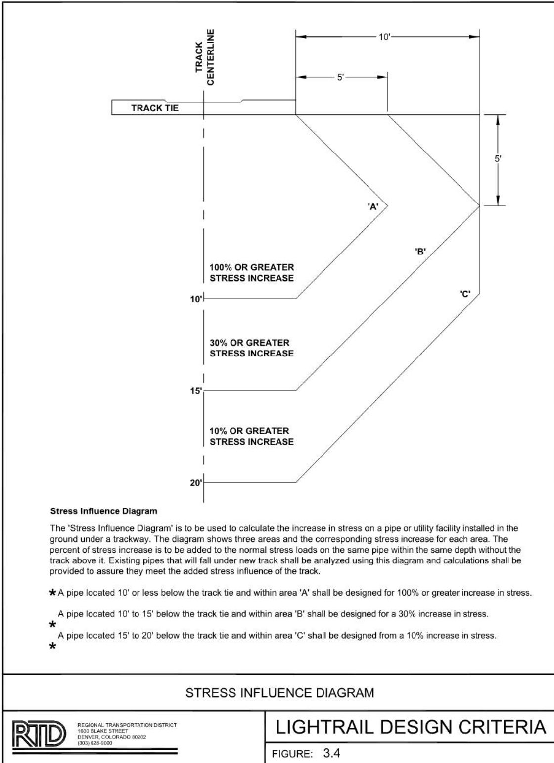
FIGURE 3 4 – STRESS INFLUENCE DIAGRAM
