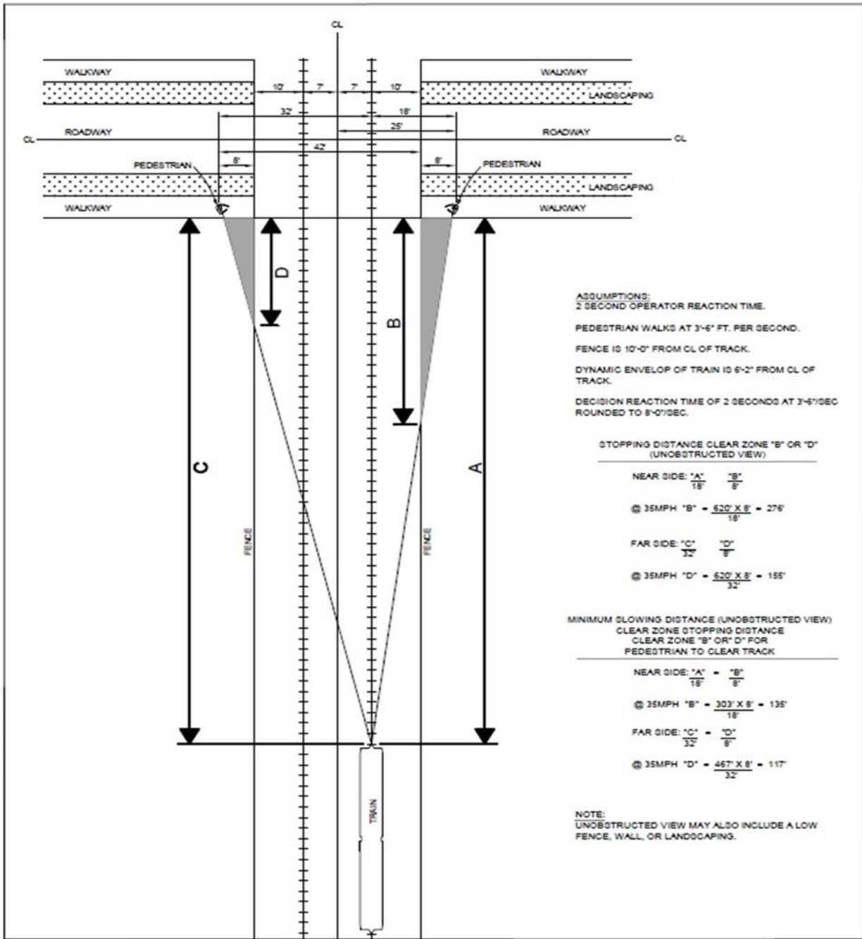
PEDESTRIAN SIGHT TRIANGLE
