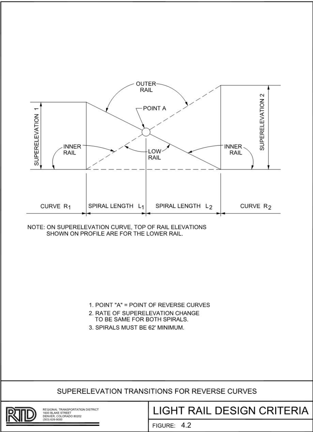
FIGURE 4.2 - SUPERELEVATION TRANSITIONS FOR REVERSE CURVES
