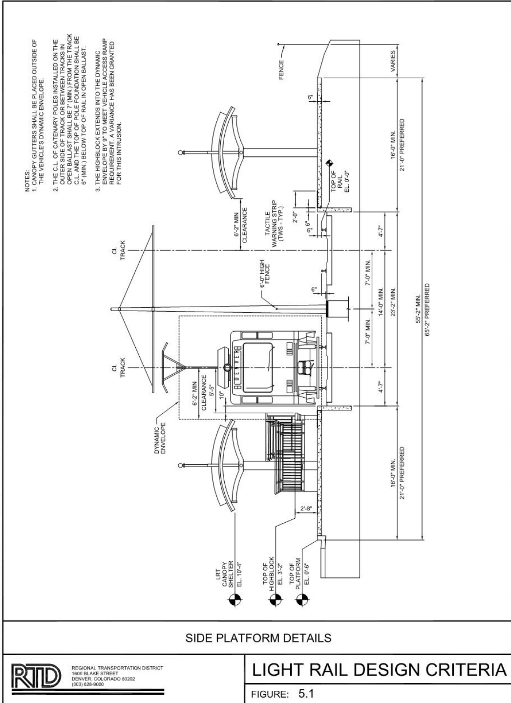
FIGURE 5.1 - SIDE PLATFORM DETAILS
