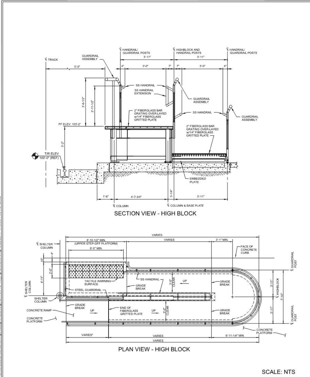
HIGH BLOCK DETAILS
