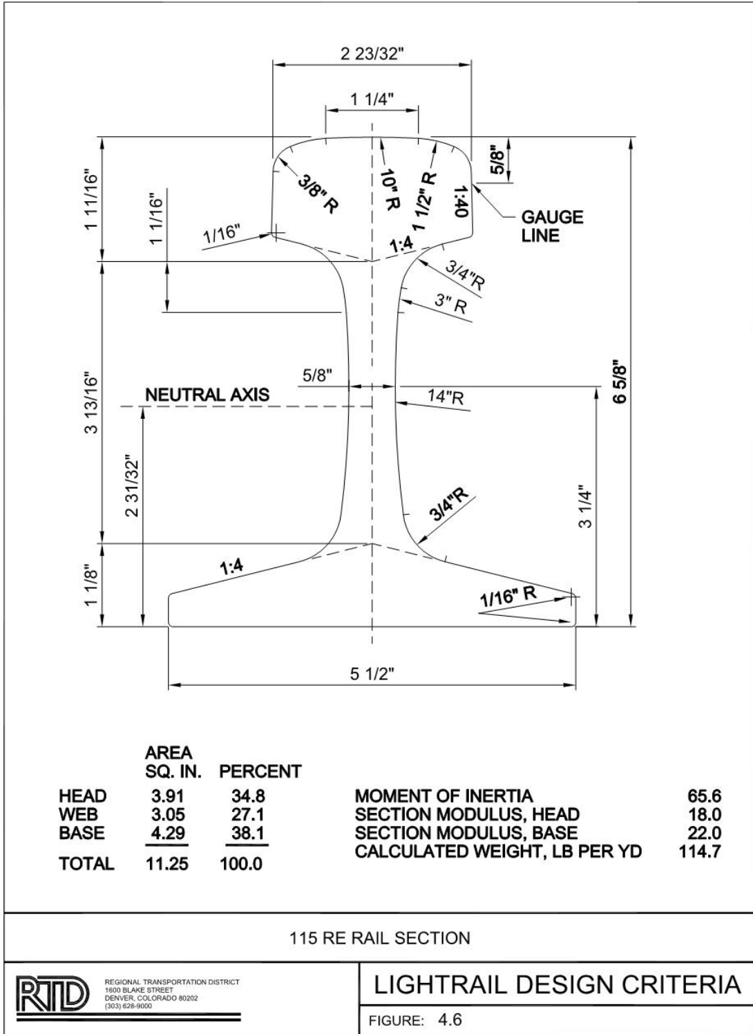
FIGURE 4.6 - 115 RE RAIL SECTION FIGURE
