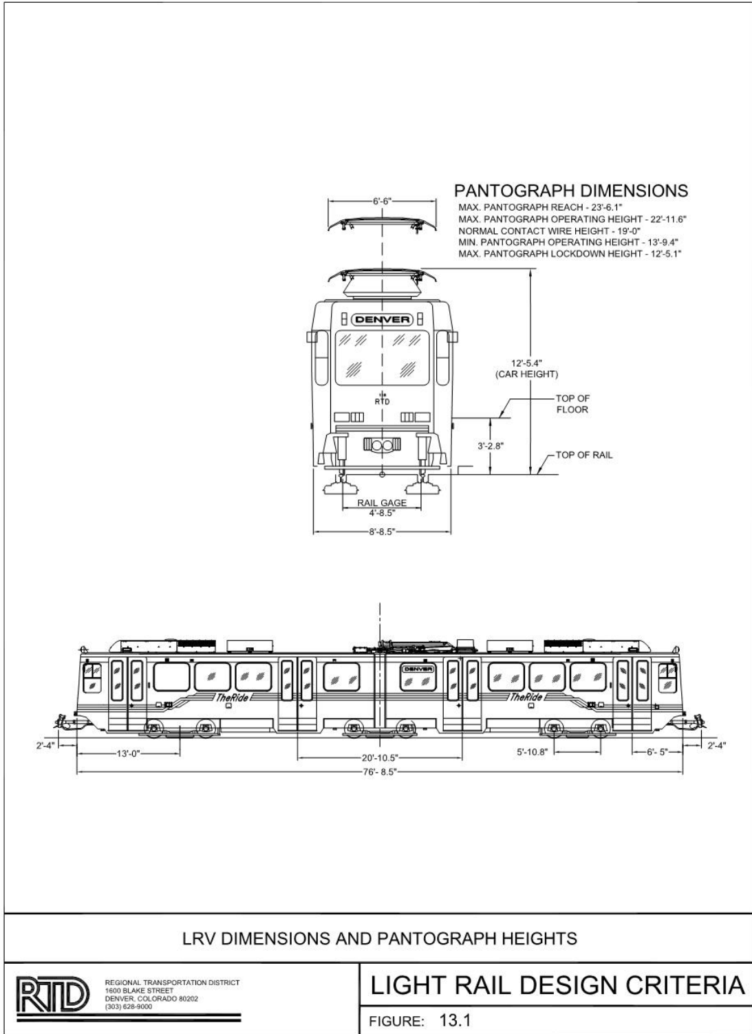
FIGURE 13.1 – LRV DIMENSIONS AND PANTOGRAPH HEIGHTS
