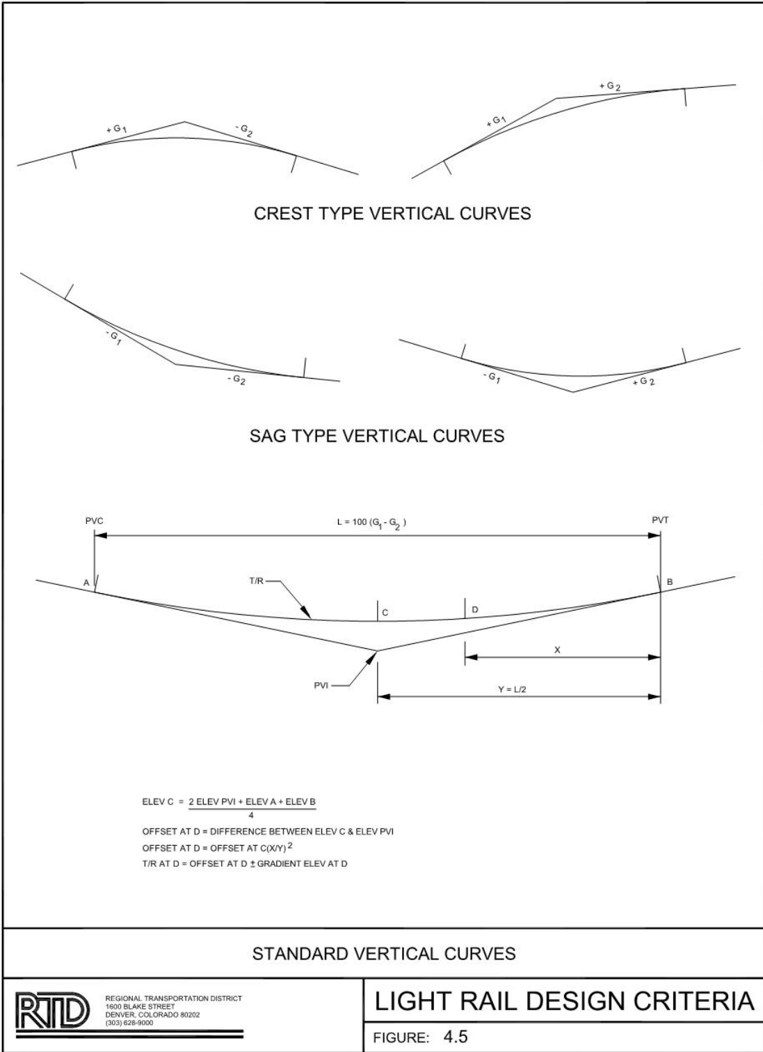
FIGURE 4.5 - STANDARD VERTICAL CURVES
