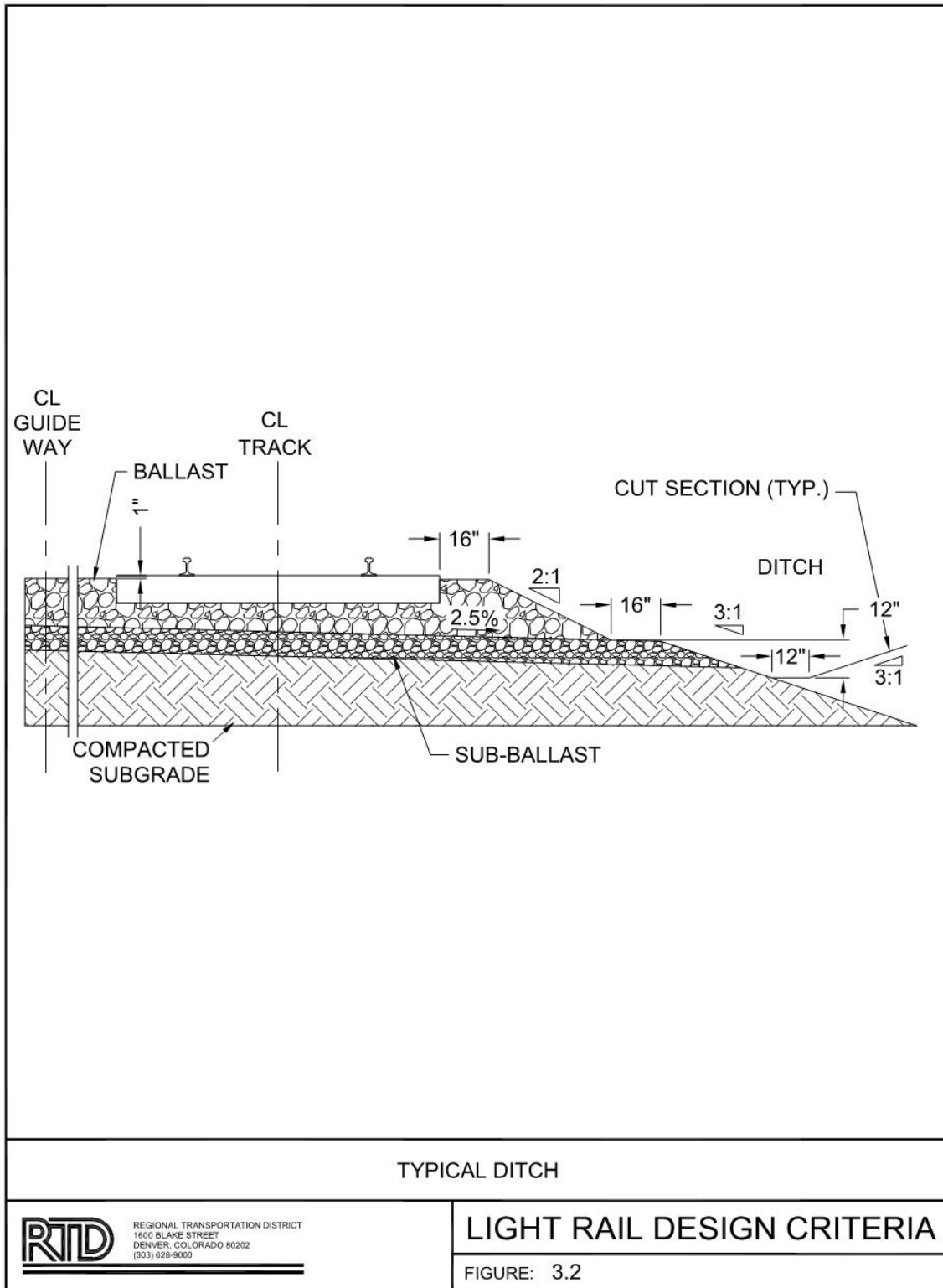
FIGURE 3 2 – TYPICAL DITCH
