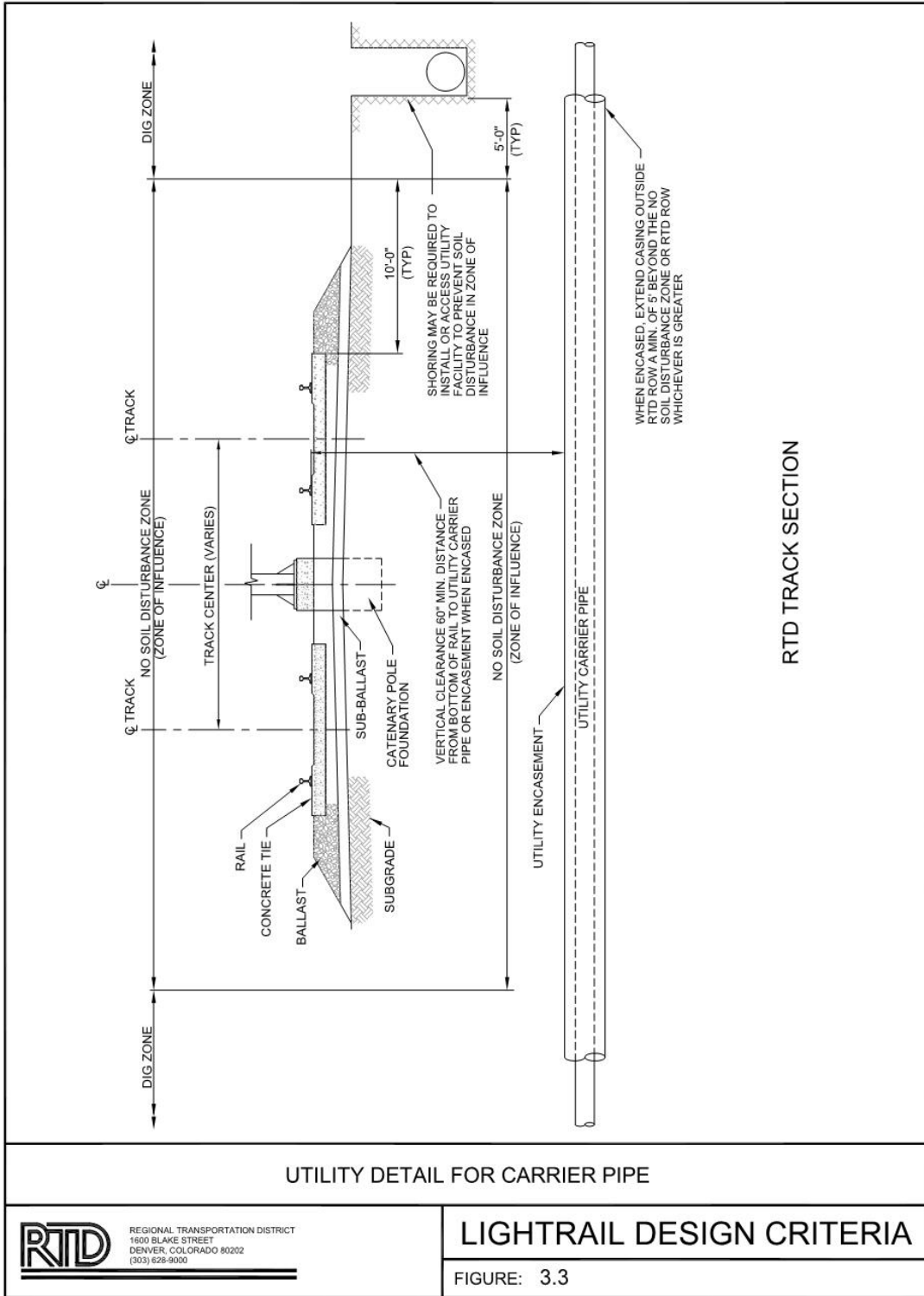
FIGURE 3 3 – UTILITY DETAIL
