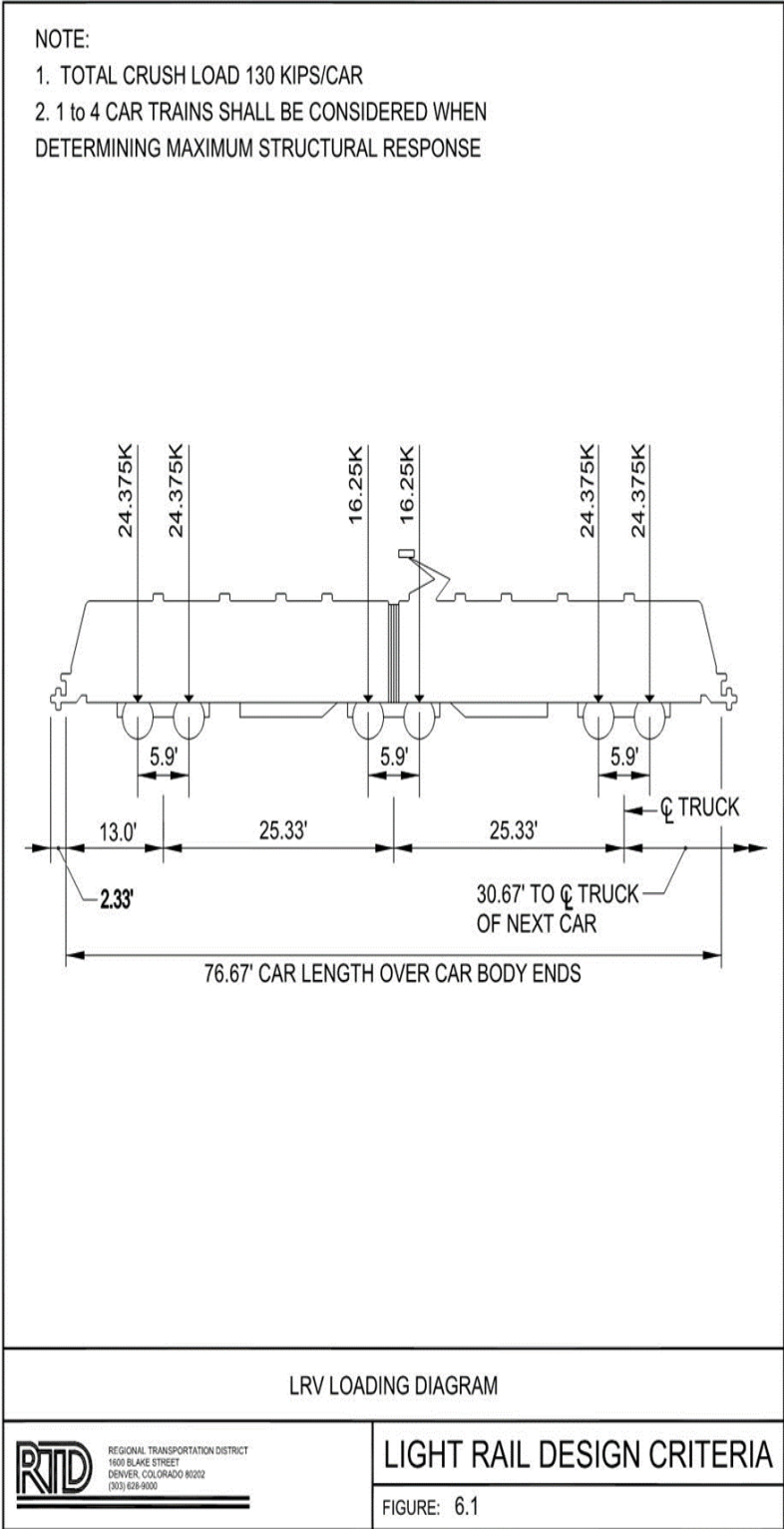
FIGURE 6.1 - LRV Loading Diagram
