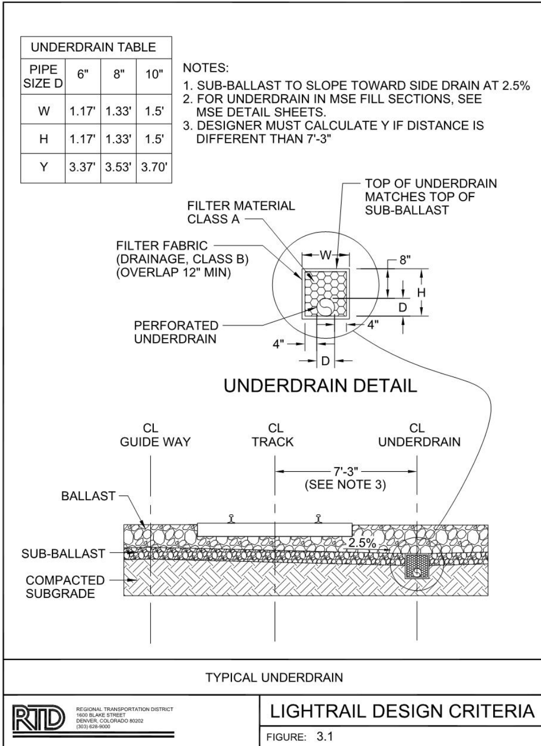
FIGURE 3 1 – TYPICAL UNDERDRAIN
