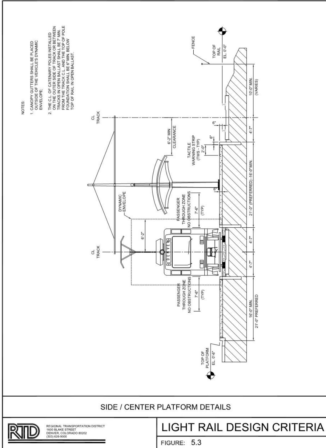
FIGURE 5.3 - SIDE/CENTER PLATFORM DETAILS
