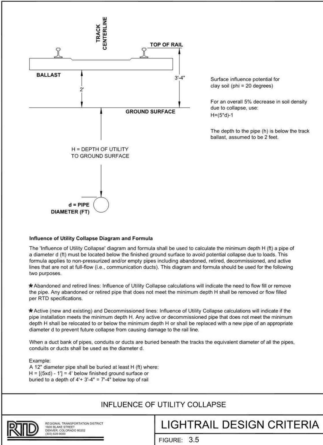
FIGURE 3.5 – INFLUENCE OF UTILITY COLLAPSE
